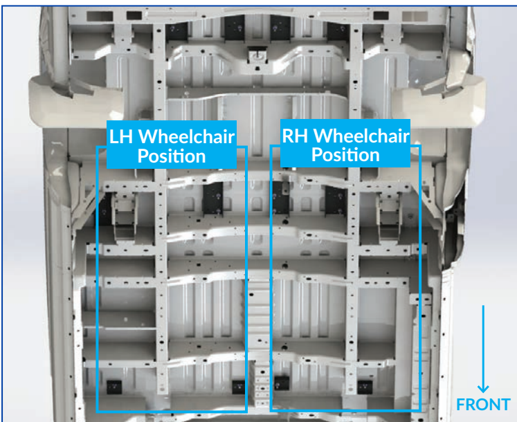
Underside view of a FORD TRANSIT VAN featuring OMNI VR brackets with Left / Right Wheelchair Positions installed
